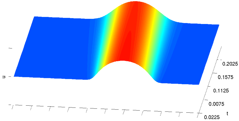
Figure 4: Evolution of the solution of (37) with u_0 defined in (40) ( L = 30 , M = 4001 and \varepsilon = 0.1 ).
