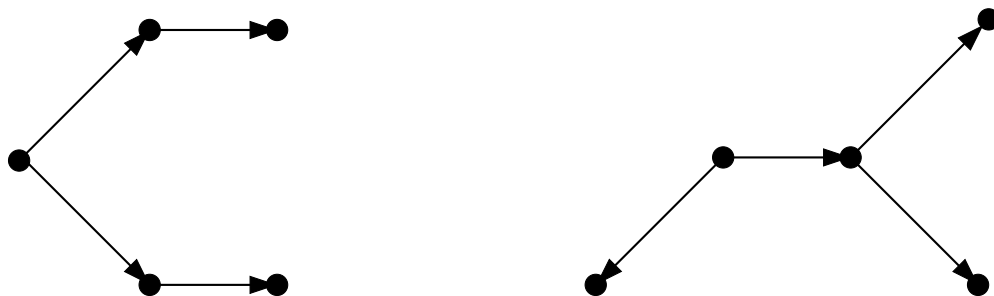
Figure 7: Two graphs having the same walk content, namely \bullet : \times 5 ; \bullet\text{---}\bullet : \times 4 and \bullet\text{---}\bullet\text{---}\bullet : \times 2 , and consequently mapped to the same point of the feature space corresponding a kernel based on the count of walks (Gärtner et al., 2003).
