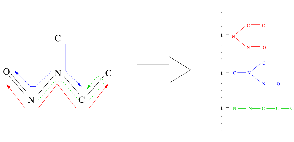
Figure 8: Illustration of the tree-structured fragment representation: a graph G (left) and an extract of its feature space representation \phi(G) (right). Note that the green tree corresponds to a walk structure.
