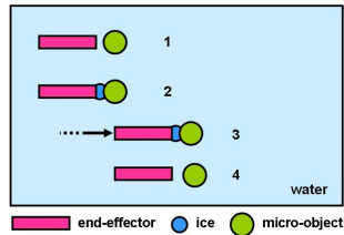
Fig. 1. Handling strategy: (1) the micro-gripper approaches, (2) an ice droplet is generated and catch the object, (3) the object is manipulated, (4) the ice thaws and the object is liberated
