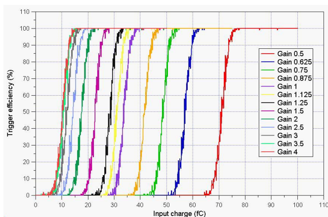
Fig. 13. S-curves for a single channel set at different preamplifier gains.
