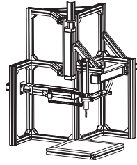
Figure 2. The Orthoglide
