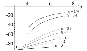
Figure 8. Influence of parameter \eta on the pressure angle \mu (in degree), with p = 50 mm and a_4 = 10 mm
