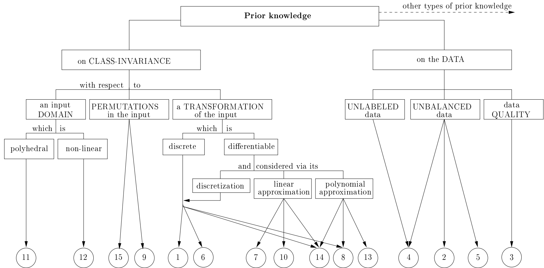
Fig. 1. Two main types of prior knowledge that can be incorporated into SVM with the corresponding methods expressed by their number given in the companion diagram of Figure 2.
