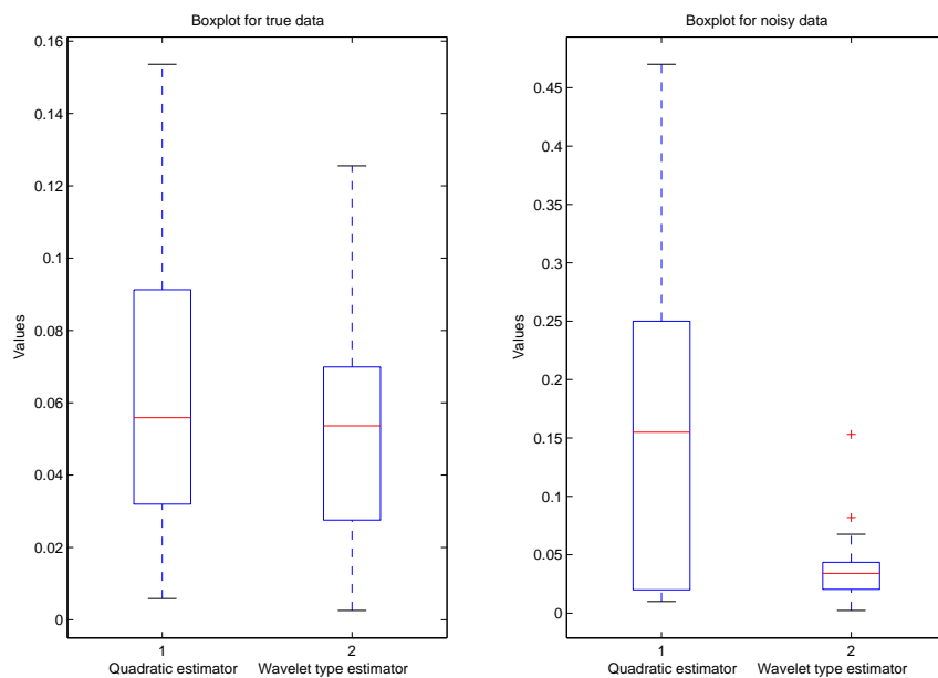
Figure 7: Boxplot for quadratic variation estimator and wavelet type estimator ( H = .4 )
