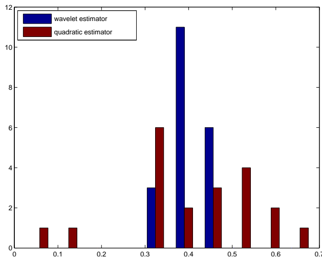
Figure 6: Comparison of Estimators Distributions with noisy observations ( H = .4 )
