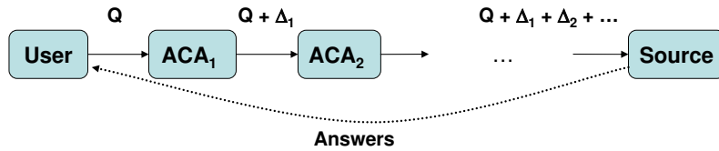
(a) Disclosing the query modifications to other ACAs and the source by keeping explicit deltas.
