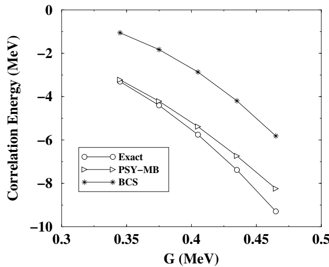
Fig. 5. Correlation energy of the ground state solution of a system of 32 particles distributed over 64 equispaced doubly degenerate levels, in function of the pairing interaction strength parameter.
