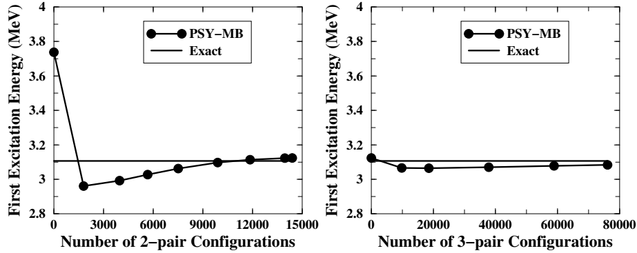
Fig. 3. Similar to Fig. 1, but for the energy of the first excited state. The value of the pairing strength parameter is G=0.345 MeV.
