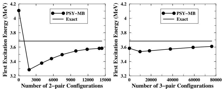
Fig. 4. The same as in Fig. 3, but for the pairing strength G=0.375 MeV.
