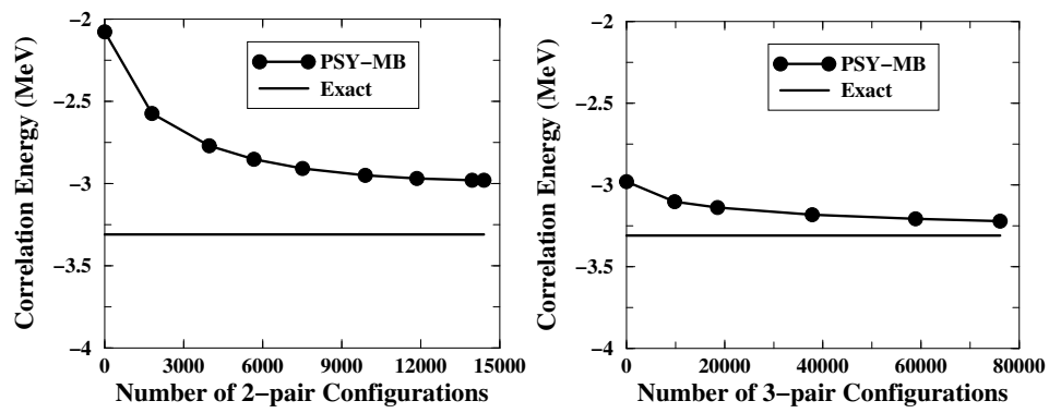
Fig. 1. Correlation energy of the ground state solution of a system of 32 particles distributed over 64 equispaced doubly degenerate levels, in function of the number of 2-pair configurations (left) and the number of 3-pair configurations (right). The value of the pairing strength parameter is G=0.345 MeV.
