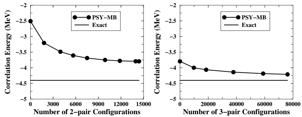
Fig. 2. Similar as in Fig. 1, but for the pairing strength G=0.375 MeV.
