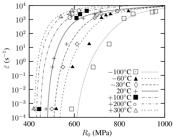
Fig. 2. Variation of the yield stress as a function of strain rate for different temperatures (lines: model, points: experiments).
