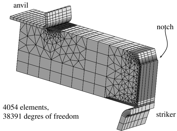
Fig. 3. Finite element mesh used for the analysis.
