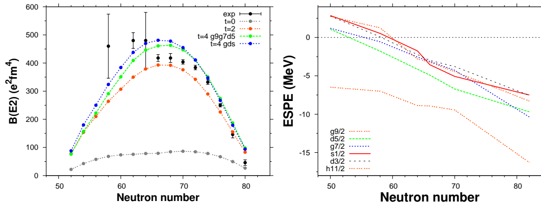
Fig. 2. left: BE2(2^+ \rightarrow 0^+) for tin isotopes; right: proton ESPE for tin isotopes.
