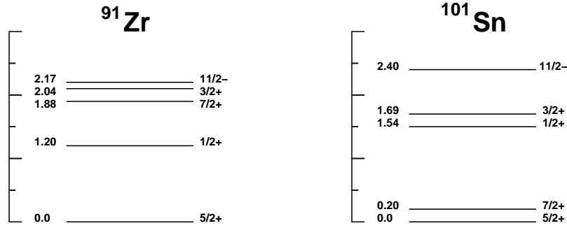
Fig. 1. Energy evolution of low-lying states between ^{91}\text{Zr} and ^{101}\text{Sn} .
