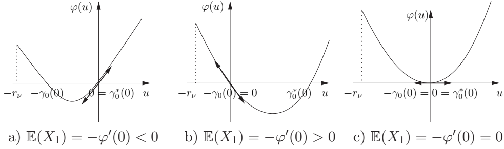
Figure 1: Graph of \varphi
