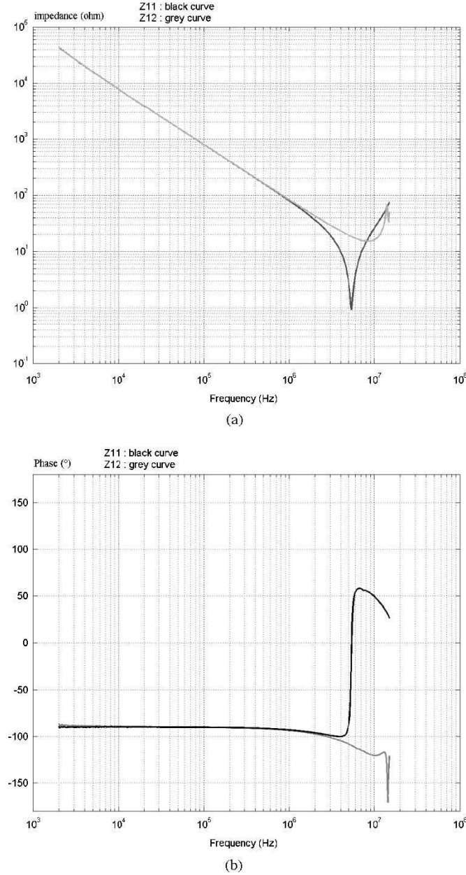
Fig. 16. Five-meter long Z_{11} and Z_{12} shielded cable CM impedance, modulus (a) and phase (b).
