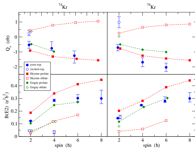
FIG. 15: Static quadrupole ( top ) moments and B(E2) values ( bottom ) for ^{74}\text{Kr} ( left ) and ^{76}\text{Kr} ( right ). The experimental values are compared to the configuration mixing calculations.
