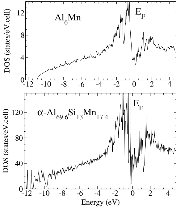
Figure 1: Ab-initio total DOS of \text{Al}_6\text{Mn} (simple crystal) and \alpha\text{-Al}_{69.6}\text{Si}_{13.0}\text{Mn}_{17.4} (approximant of icosahedral quasicrystals) [11, 12].
