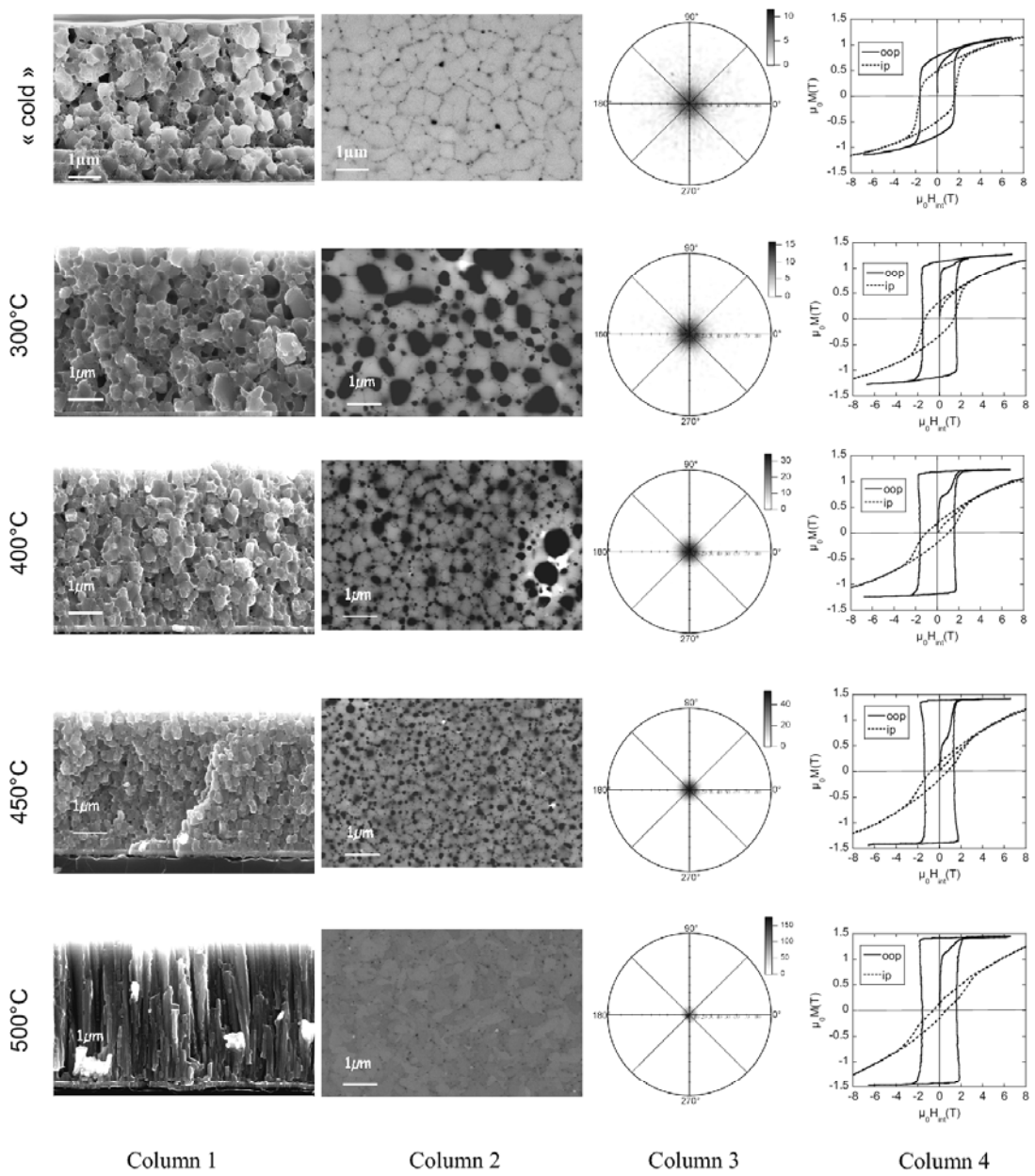
FIG. 1. Comparison of the evolution in structural and magnetic properties of NdFeB films as a function of deposition temperature (note all films were annealed at 750°C for 10 minutes). Column 1 : Fractured cross sections imaged with an in-lens detector Column 2 : Polished plane views imaged in QBSD mode Column 3 : XRD pole figure of (006) diffraction peak of \text{Nd}_2\text{Fe}_{14}\text{B} Column 4 : In-plane (ip) and out-of-plane (oop) hysteresis loops and the initial oop magnetization curves (oop loops were corrected with a demagnetization factor N = 1 ).
