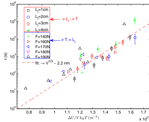
Figure 9: Logarithm of lifetimes as a function of the dimensional factor \Delta U/(Vk_B T) predicted by eq. 2 for different values of L_i , F and T . The slope of the best fit \log \tau \propto \Delta U/k_B T (dashed line) gives an estimation of the characteristic length scale V^{1/3} \sim 2.2 nm. Data points without error bars correspond to non-averaged measurements obtained when varying temperature with L_i = 2 cm and various fixed values of F .
