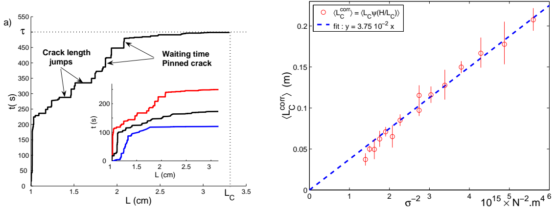
Figure 6: a) Typical stepwise growth curve for a creep experiment with an initial crack length L_i = 1\text{cm} submitted to a constant load F = 270\text{N} . The lifetime of the sample is \tau = 500\text{s} and the critical length L_c = 3.3\text{cm} . In insert, a strong dispersion is observed in crack growth profile and in lifetime for 3 creep experiments realized in the same conditions. b) Critical length of rupture L_c as function of the inverse square of the applied stress 1/\sigma^2 . The dashed line represents the best linear fit y = K_c^2 x . Its slope permits us to estimate the critical stress intensity factor K_c . Note that we introduce the finite height corrections in the critical length L_c^{corr} .
