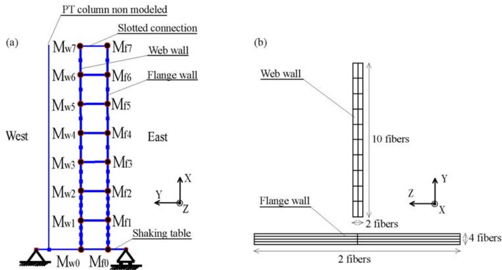
Figure 2.2. (a) Finite element mesh and concentrated masses and (b) fibers in a given section.
