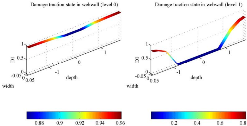
Figure 2.11. State of damage in concrete due to traction for the modified structure at levels 0 and 1 considering new material and damping data and the continuity of steels (EQ1).
