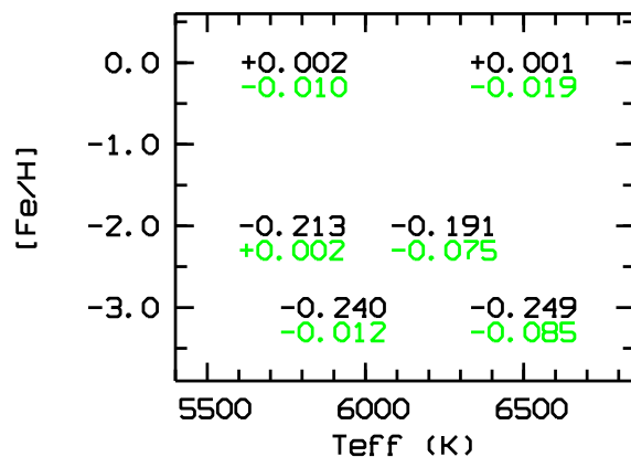
Fig. 2. 3D abundance corrections: each correction is located according the parameters ( T_{\text{eff}} and [Fe/H]) of the related model; the models have very similar gravity ( \log g in between 4.44 and 4.50). Black numbers depict the 3D-1D LHD differences, grey (green in colour) ones the 3D-1D internal model differences.
