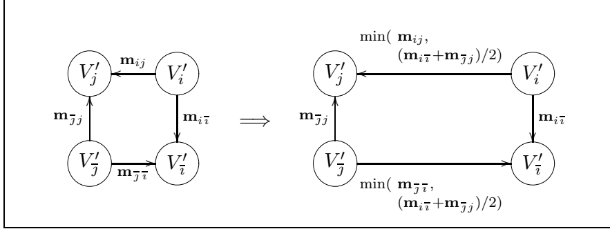
Figure 8. Additional propagation step performed by the strong closure.
