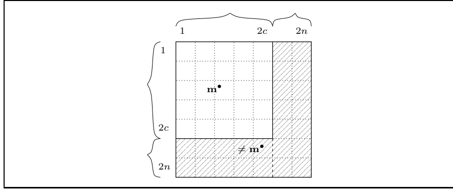
Figure 10. A matrix equal to \mathbf{m}^\bullet except for the last 2(n - c) lines and columns.
