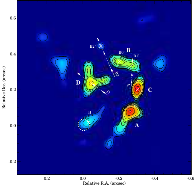
Fig. 2. H-band map of IRC+10216, where only the highest spatial frequencies of the brightness in the Fourier space have been kept. The contour levels are 80, 50, 20, 10, 8, 5, 2, 1 and 0.5% (this minimum level being the estimated noise). The dotted circle is the assumed star position, as in Fig. 1. Main clumps are indicated by the labels A to D, and some sub-features by the smaller labels. The positions of these clumps are shown by the white crosses. Estimated trajectories (from the results of Tuthill et al. 2000) for some clumps with respect to clump A are also shown (see text for details).
