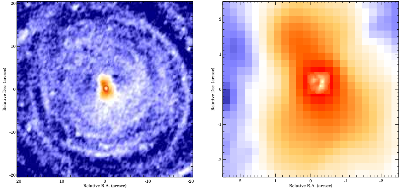
Fig. 10. View of the IRC+10216 CSE inner morphology. Left panel shows the closest structures around the center detected in V-band. Right panel shows the V-band image core, on which has been superposed the NACO H-band image. The overlapping has been done by assuming that the NACO and FORS peak brightness are found at the same location.
