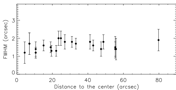
Fig. 9. Relation between the thickness of the shells and their distance to the center.
