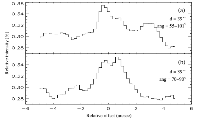
Fig. 7. Comparison of the profile of the shell d estimated as in MH00 (top panel) with its profile derived by our more complex method (bottom panel, see text for details). The distances to the center, d , of the shells and the ranges of their azimuthal angles from north, ang , are given. The relative intensity is with respect to the central peak brightness of the original image.
