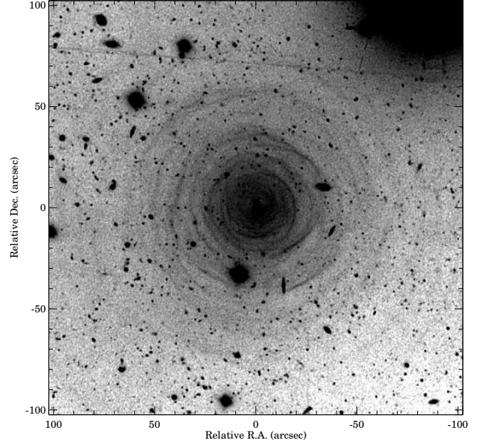
Fig. 3. FORS1 deconvolved V-band image of IRC+10216. North is up and East is left.
