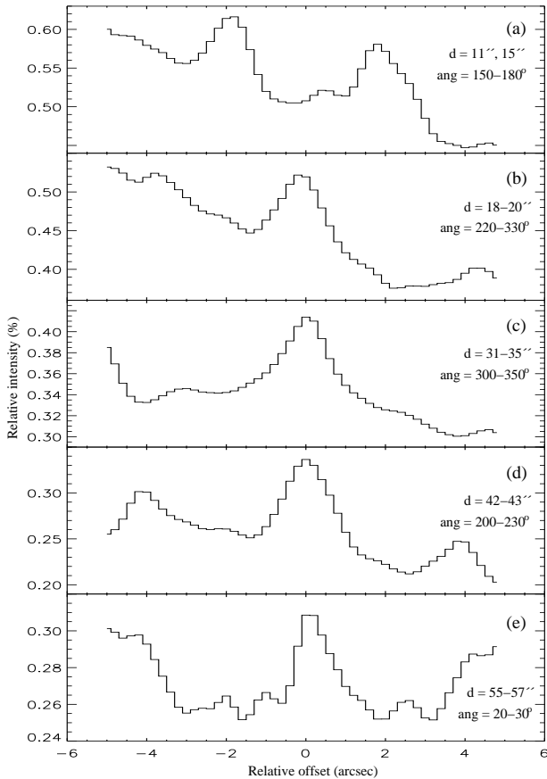
Fig. 8. Profiles of some shells considering their non-concentric nature (see text for details). There are two shells in the panel (a) and one in the others. The given parameters follow the same definitions as in Fig. 7. The ranges in the shell distances to the center, d , are due to their non-concentric nature.
