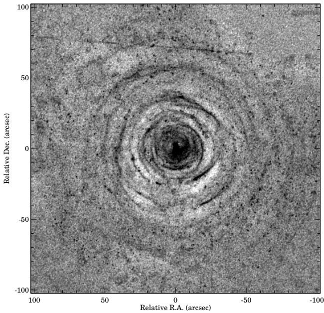
Fig. 4. Deconvolved V-band image after subtraction of the halo of the CSE and removing of most stars and galaxies.
