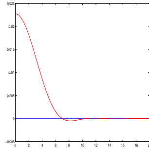
FIGURE 1. Profile of the kernel K_0
