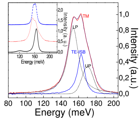
FIG. 2: Normalized photovoltage spectra (spectral resolution of 8 \text{ cm}^{-1} , at 78\text{K} ) for \theta = 75^\circ . The solid lines labelled with TM and TE-ISM represent the spectra collected with TM- and TE-polarized light respectively. The two peaks in dashed lines, labelled LP and UP, are the Lorentzian and Gaussian functions, respectively, used in the fitting procedure explained in the text. The result of the three curve fit is shown by the dotted line. Inset: photovoltage spectra with different incident angles ( 67.7^\circ solid line, 76.3^\circ dotted line, 81.2^\circ dashed line).
