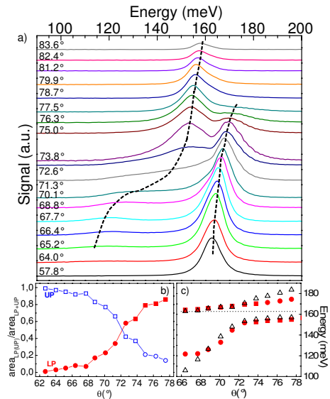
FIG. 3: a) Photovoltage spectra (at 78 K) obtained with TM-polarized incident radiation, after subtraction of the TE peak, presented as a function of the propagating angle within the cavity. The spectral resolution is 8 \text{ cm}^{-1} and the spectra are offset each other for clarity. The dashed lines are guides for the eye. b) Areas of the UP (open symbols) and LP (full symbols) peaks, normalised to the total area, as a function of the internal angle. Squares (circles) represent values obtained using a Lorentzian (Gaussian) function in the fit. c) Energy position of the photovoltage peaks as a function of the incident angle of the radiation (squares for Lorentzian functions, circles for Gaussian functions), compared with the results of the transfer matrix calculations (open triangles). The dashed line shows the energy of the bare ISB transition.
