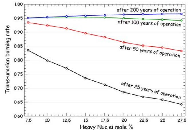
Fig.9. Burning rate of all the transuranic elements after different operation times, as a function of the HN proportion
