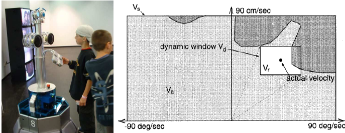
Fig. 9. The Minerva (top-left), Rhino (top-right) and Robox (bottom-left) tour-guide robots rely upon the Dynamic Window approach for collision avoidance (bottom right, source [5]).
