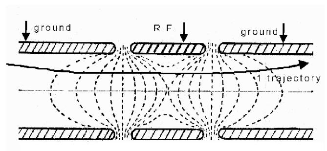
Figure 11. Equipotentials due to the R.F. applied. Their integrated effects depend on the ion positions inside the “inflating”.
