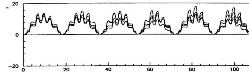
With corrections each 18 m (12 quadrupoles) and earth magnetic field
