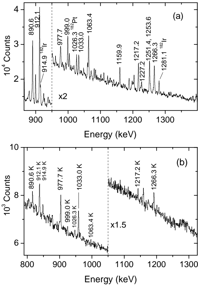
Fig. 5. High-energy section of the (a) \gamma -ray and (b) electron singles spectra corresponding mainly to the ^{182}\text{Ir} \rightarrow ^{182}\text{Os} decay.
