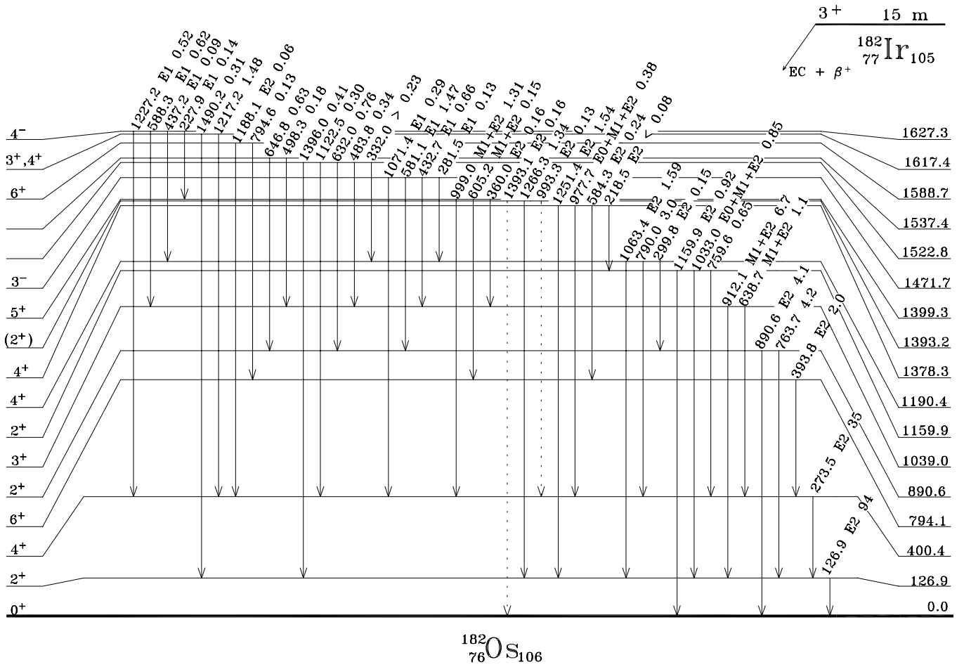
Fig. 1. Level scheme for ^{182}\text{Os} from ^{182}\text{Ir} decay (lower part). Total intensities, I(\gamma+e) , per 100 parent decays and some multiplicities are indicated.
