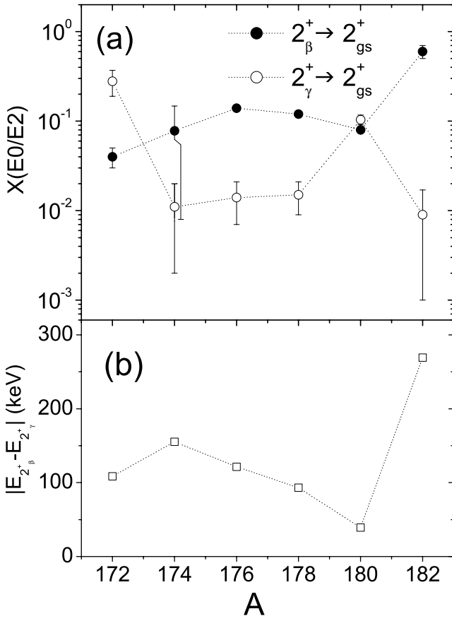
Fig. 7. Systematics of (a) the X(E0/E2) strengths for the 2_{\beta}^{+} \rightarrow 2_{gs}^{+} and 2_{\gamma}^{+} \rightarrow 2_{gs}^{+} transitions and (b) the absolute energy difference between the 2_{\beta}^{+} and the 2_{\gamma}^{+} states in the A = 172 - 182 Os isotopes.
