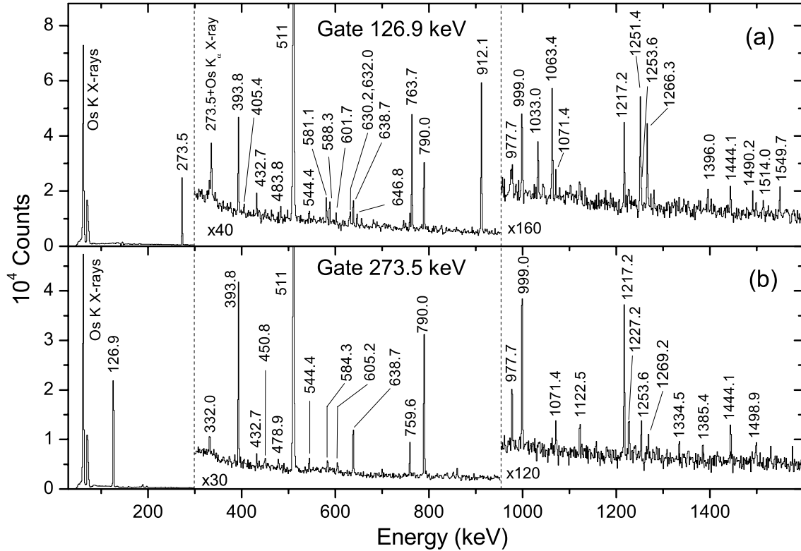
Fig. 3. \gamma -ray coincidence spectra gated on the (a) 126.9 keV and (b) 273.5 keV \gamma -rays belonging to the ^{182}\text{Ir} \rightarrow ^{182}\text{Os} decay.
