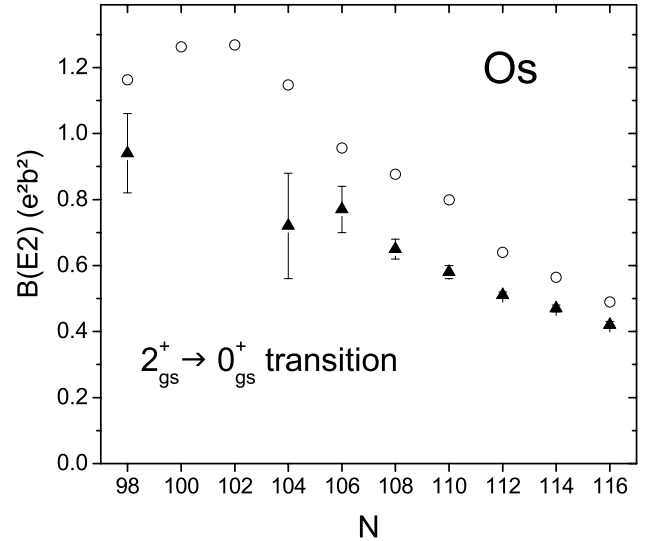
Fig. 10. Experimental (full symbols) and predicted (open symbols) B(E2) values of the 2_{gs}^+ \rightarrow 0_{gs}^+ transitions in the even-even ^{174-192}\text{Os} nuclei.
