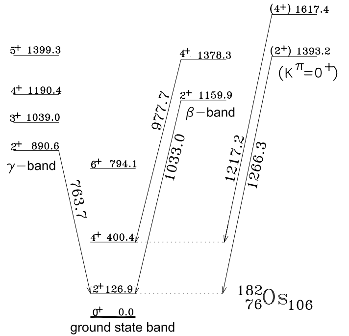
Fig. 6. Ground state band, \gamma -band, \beta -band, and a proposed second excited K^\pi = 0^+ band of ^{182}\text{Os} , as observed in the present work. The transitions, for which E0 components were assigned, are indicated.
