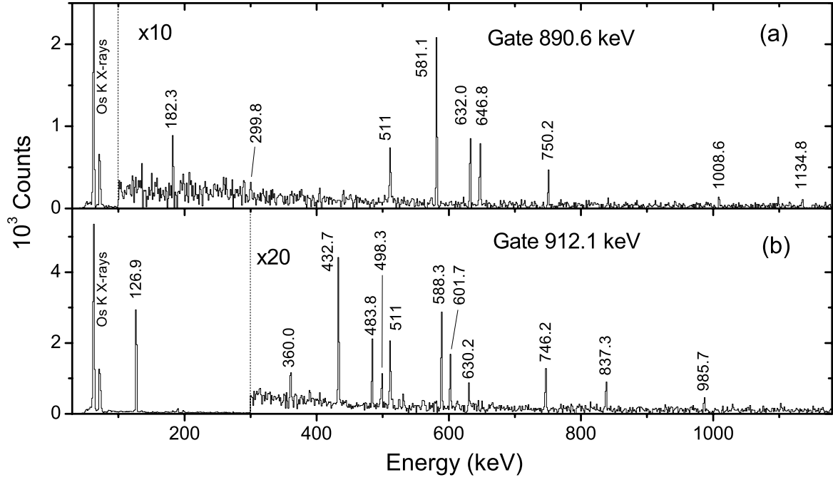
Fig. 4. \gamma -ray coincidence spectra gated on the (a) 890.6 keV and (b) 912.1 keV \gamma -rays belonging to the ^{182}\text{Ir} \rightarrow ^{182}\text{Os} decay.
