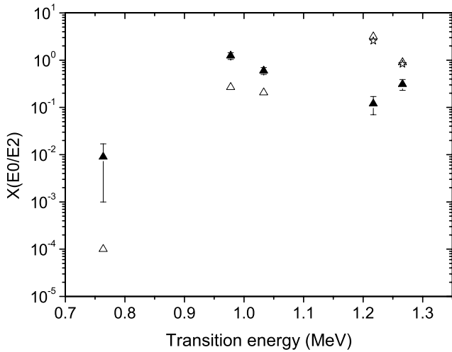
Fig. 11. Experimental (full symbols) and predicted (open symbols) X(E0/E2) values for the five highly converted transitions of ^{182}\text{Os} .
