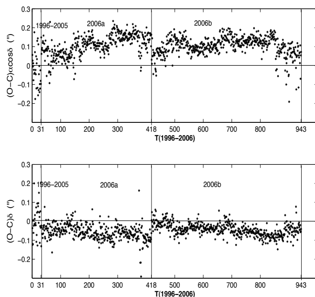
Figure 4. Plots of residuals in right ascension and declination of the absolute positions of Triton, derived from the comparison of our all observations to the IMCCE ephemeris vs. time T(1996 - 2006)
