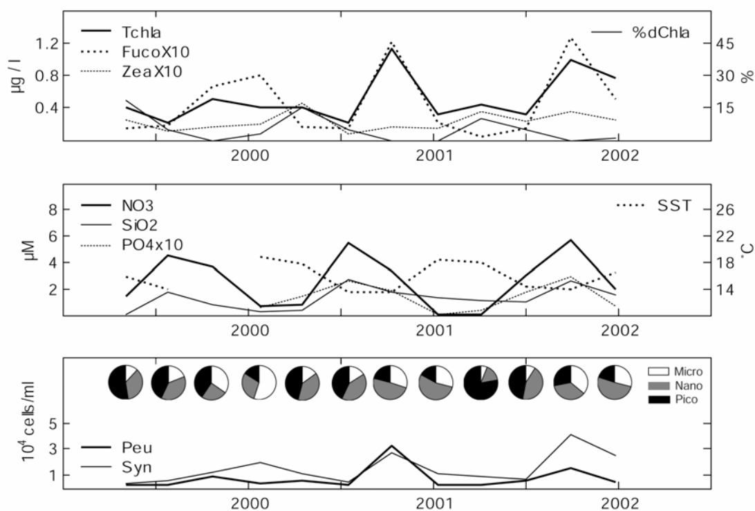
Fig. 3.- Time variations detected by GeP&CO cruises in NADR. Plots correspond to average values of \sim 12 observations at the sea surface in this province for each cruise. From top to bottom: first panel, total chlorophyll a (Tchl a, bold line), percentage of divinyl-chlorophyll a (%dChla, thin line), concentration of fucoxanthin (Fuco, bold dotted line, multiplied by 10) and zeaxanthin (Zeax, thin dotted line, multiplied by 10); second panel, sea surface temperature (SST, bold dotted line), concentrations of nitrate (NO 3 , bold line), silicate (SiO 2 , thin line) and phosphate (PO 4 , thin dotted line, multiplied by 10); third panel, contribution of picoplankton (black), nanoplankton (gray) and microplankton (white) to total chlorophyll a (pie charts), cell numbers of picoeucaryotes (Peu, bold line), and Synechococcus (Syn, thin line).
