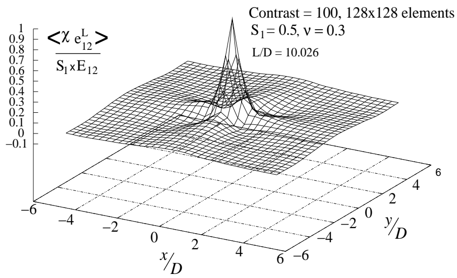
FIG. 1 – Normalized correlation function \langle \chi e_{12}^L \rangle .
