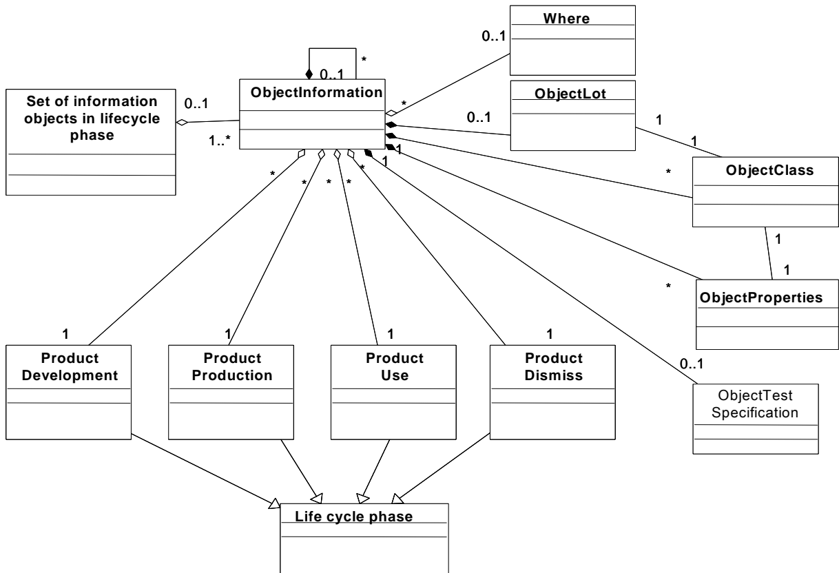
Figure 5. The Object Information model
