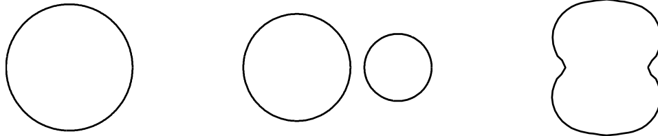
Figure 5: The disk probably minimizes \lambda_3 (left); two disks which probably minimize \lambda_4 (center); a domain candidate to minimize \lambda_5 (right).
