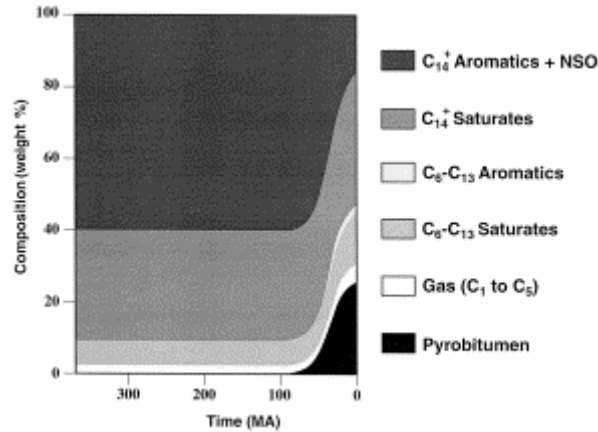
Fig. 11. Numerical modeling of oil composition as a result of natural thermal cracking as a function of time.
