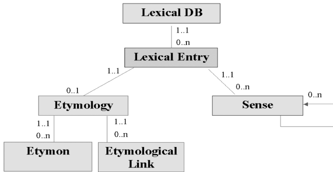
Figure 2: The LMF metamodel and the etymological extension
