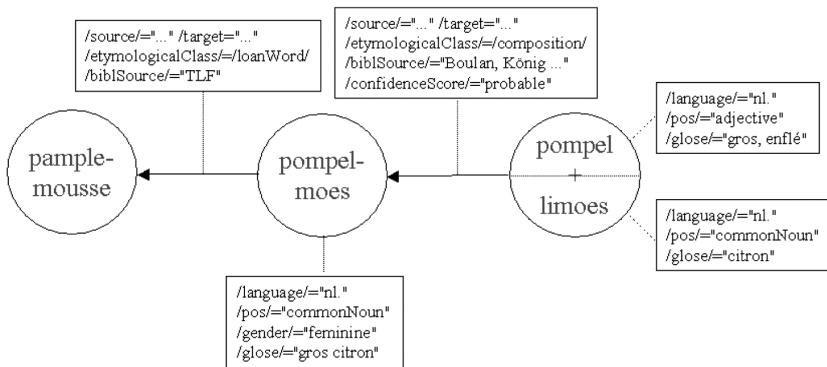
Figure 4: Etymological data structure for pamplemousse (TLF)
