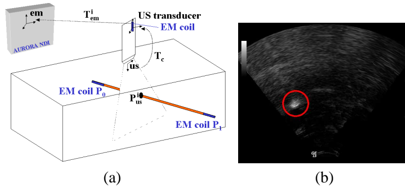
Figure 3. US/EM spatial calibration (a) experimental set up for a position i of the US transducer. (b) an US image of the pointer.
