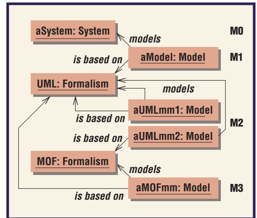
Figure 2. Four-layer UML formalism instantiating Figure 1's basic model. M0 is the modeled system layer; M1 describes the user models; M2 is the UML metamodel layer; and M3 is the meta-metamodeling layer, which defines metalanguages such as MOF for the M2 level.
