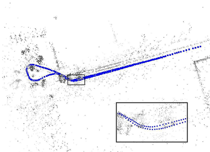
Figure 3. Top view of a complete reconstruction in an urban environment. The distance covered is about 200 meters long including a half-turn. More than 8.000 3D points have been reconstructed for 240 key frames.
