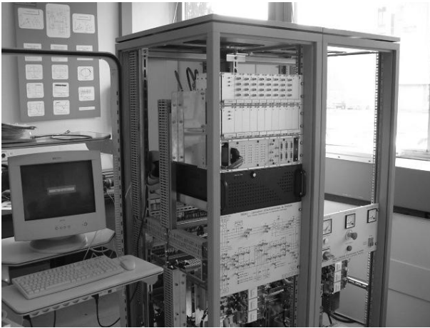
Figure 5: Experimental bench
