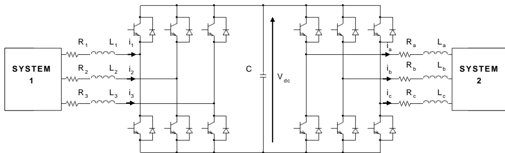
Figure 3: AC/DC/AC three phase converter used as power interface
