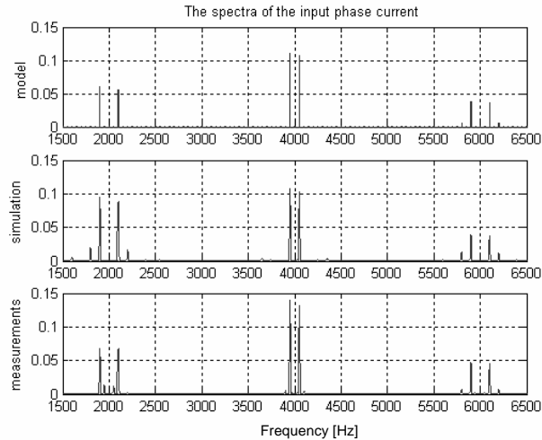
Figure 7: AC current spectrum from the network side; theoretical, simulation, and experimental results
