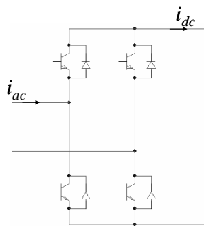
Figure 1: a simple switching process
