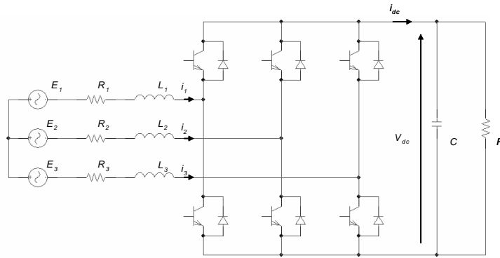
Figure 4: AC/DC converter
