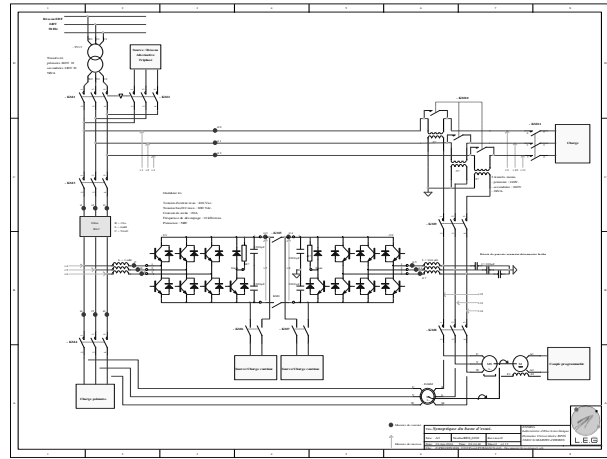
Figure 6: Experimental bench description
