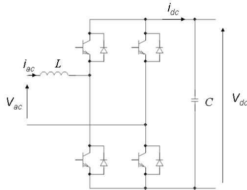
Figure 2: a simple converter structure
