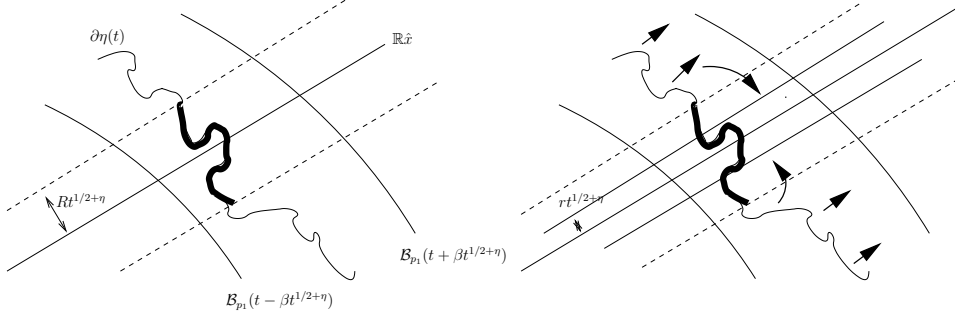
FIGURE 1. On the left hand side, \text{Shadow}(x, t, R t^{1/2+\eta}) : the strong are in bold. On the right hand side, the evolution of the weak: to enter \text{Cyl}(x, r t^{1/2+\eta}) , it has to cross a gap of order (R - r)t^{1/2+\eta} .
