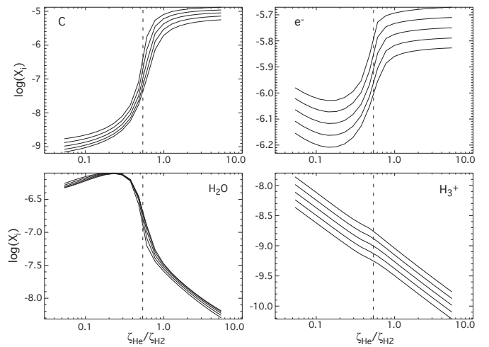
Fig. 5. Abundances of C, e^- , \text{H}_2\text{O} and \text{H}_3^+ as a function of \zeta_{\text{He}}/\zeta_{\text{H}_2} and for five different values of \zeta_{\text{He}} (solid lines). The vertical dashed line indicates the standard value of \zeta_{\text{He}}^0/\zeta_{\text{H}_2}^0 .
