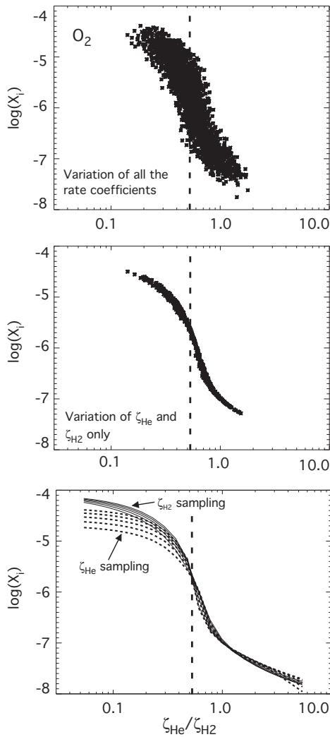
Fig. 4. Abundance of \text{O}_2 as a function of \zeta_{\text{He}}/\zeta_{\text{H}_2} at 10^7 yr. The upper and middle panels represent the abundance computed with the random distribution of all the rate coefficients and of \zeta_{\text{He}} and \zeta_{\text{H}_2} only, respectively. The solid lines in the lower plot have been computed using one value of \zeta_{\text{He}} for each line and varying \zeta_{\text{H}_2} , while the dotted lines have been computed using one value of \zeta_{\text{H}_2} for each line and varying \zeta_{\text{He}} . The vertical dashed line indicates the standard value of \zeta_{\text{He}}^0/\zeta_{\text{H}_2}^0 .
