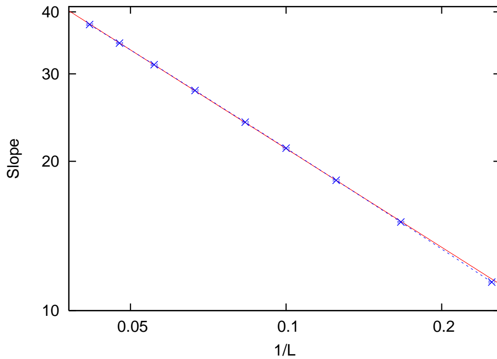
Figure 6: Slope of the domain-wall free energy of the Gaussian random-bond Ising model as a function of 1/L .
