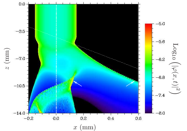
FIG. 5: (Color online) Contour plot depicting the time evolution of the envelope of |\varphi(x, t)|^2 on a logarithmic scale as a function of x and of z(t) = z_0 - \dot{z}_0 t - \frac{1}{2} g t^2 . The atom is falling in the gravity field in the presence of the two trapping potentials with U_0 = 30 \mu\text{K} , U_1 = 10 \mu\text{K} , w_0 = 0.2 mm and w_1 = 0.3 mm. The two guides cross at the height z_c = -4 mm with an angle \gamma = 0.12 rad, and the oblique guide is switched on at t_0 = 28.6 ms. The vertical and oblique dotted white lines reveal the directions of propagation of the laser beams. The two white arrows point to the location of the maximum probability density at the height z = -10 mm. The initial level is here v_0 = 6000 .
