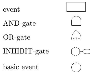
Fig. 1. Fault Tree Symbols
