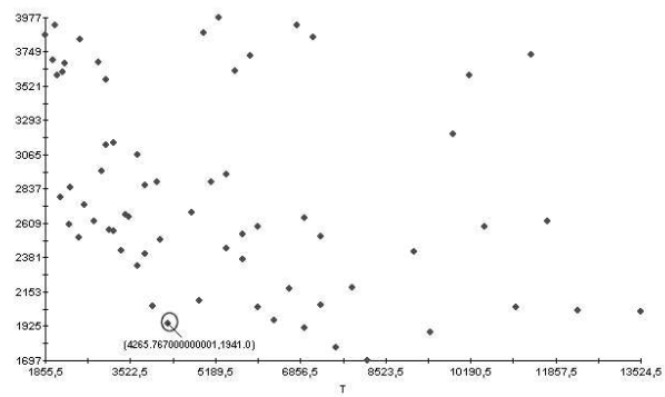
Figure 3: Horizontal DWT exploration results (Virtex) - slices vs time
