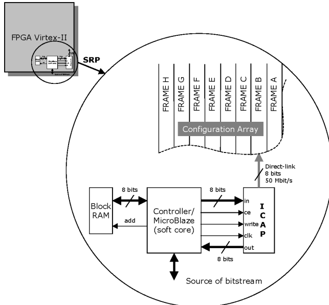
Figure 4 Schematic view of the self-reconfigurable platform SRP. The ICAP port is directly connected to the configuration array. It can partial reconfigure the different frame of configuration. The configuration controller can be a MicroBlaze soft core. The bitstream file can be provided from outside or inside the circuit. The BlockRAM can be used like configuration memory
