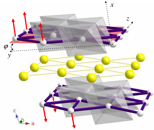
FIG. 6: The orientation of the hard axis z and the easy axis x relative to the triangular Ni layers. The ab plane is highlighted in the top layer. The z axis is parallel to the b direction in the crystal; the angle between the ab plane and the y axis is \varphi \approx 10^\circ . The spin directions are indicated by red arrows.
