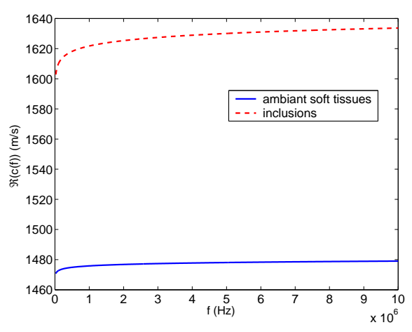
Figure 5: Evolution of the sound speed versus f .
