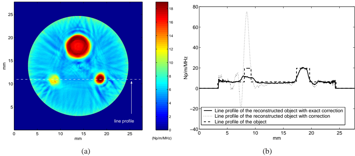
Figure 10: Reconstruction using log spectral difference technique with exact correction of the scattering effects (a) and line profile (b).
