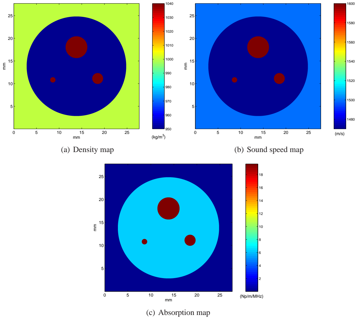
Figure 1: Cylindrical academic computer phantom.
