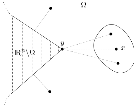
Figure 1: Analogy with the Euclidian distance.
