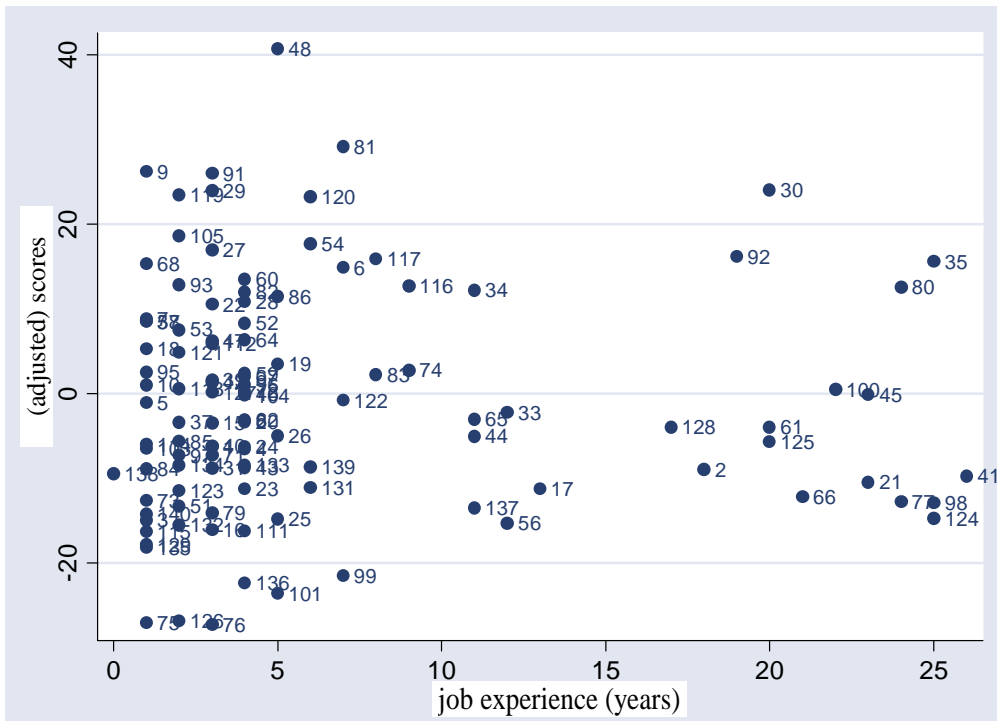
Figure A1.1: Partial scatter plot of final test scores (class average) on teacher job experience, for classes taught by civil servant teachers, grade 2
