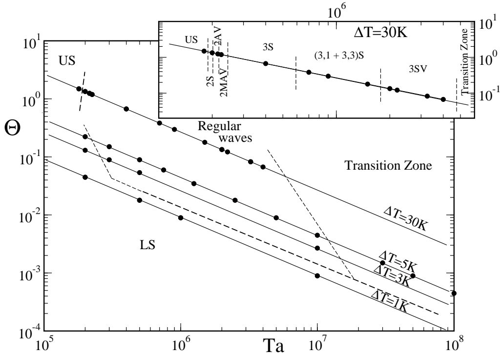
FIGURE 2. Summary of the regimes for air with Prandtl number of 0.7 as obtained by the numerical model. The solid lines show the temperature differences investigated in this paper and previously by Maubert & Randriamampianina (2002) and Maubert & Randriamampianina (2003). The dots on the lines for \Delta T = 1, 3, 5K correspond to cases discussed in the earlier papers while the dots on the line for \Delta T = 30K show the cases discussed here. The dashed line indicates the transition from the symmetric regimes to regular waves, and the dotted line indicates the transition from regular waves to irregular flow. The line for \Delta T = 30K is shown again enlarged in the insert to identify the different regimes observed in this study.
