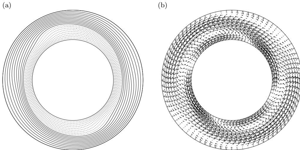
FIGURE 5. Horizontal cross-sections at mid-height of a 2S flow at Ta = 200,000 . (a) Temperature contours and (b) the horizontal velocity field.
