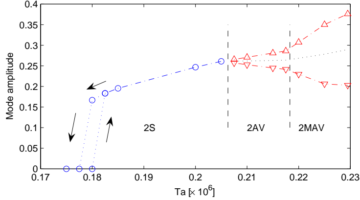
FIGURE 3. The amplitude of the dominant azimuthal mode, m = 2 , at mid-radius. The dash-dotted lines indicate the global maximum and minimum of the amplitude. The dash-dotted lines in the 2MAV regime denote the largest amplitude minimum and the smallest amplitude maximum of all the extreme values in each vacillation cycle, while the dotted lines in 2MAV show the average of the amplitude minimum and maximum for all vacillation cycles, respectively. The dotted line in the 2AV regime shows the averaged amplitude.
