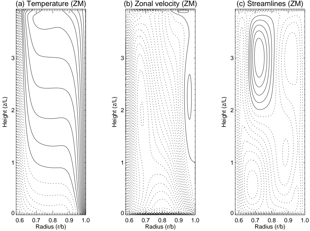
FIGURE 12. Zonal mean fields for the typical wave-3 simulation at Ta = 1.5 \times 10^6 using air as the working fluid. (a) Temperature (contour interval = 0.1, normalised to an imposed temperature difference of \pm 1.0 ), (b) zonal velocity V_\phi (contour interval = 0.25 dimensionless units) and (c) meridional stream function (contour interval = 0.01 dimensionless units).
