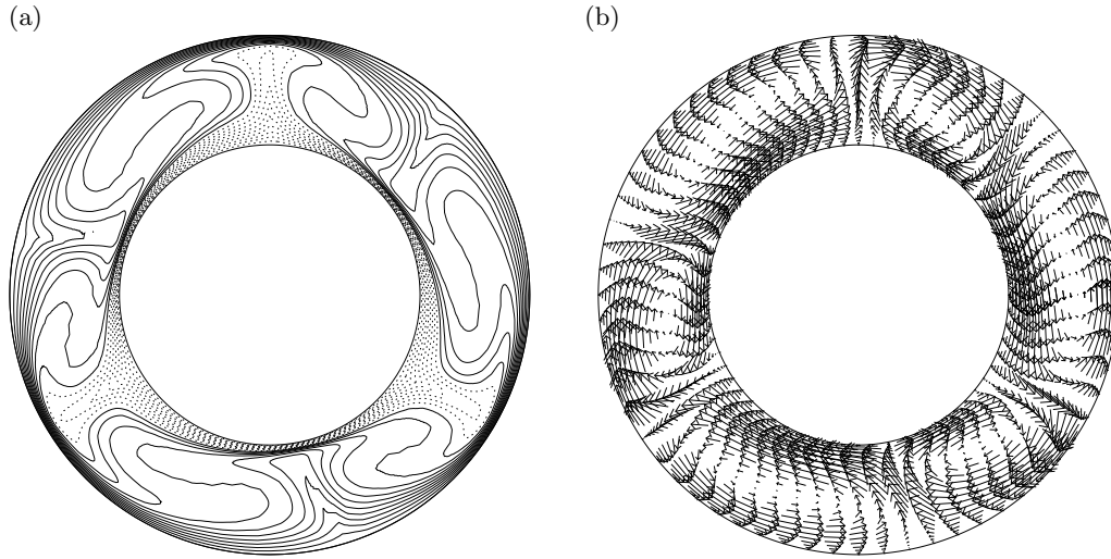
FIGURE 10. Horizontal cross-sections at mid-height of a wave-3 flow at Ta = 1.5 \times 10^6 . (a) Temperature contours and (b) the horizontal velocity field.
