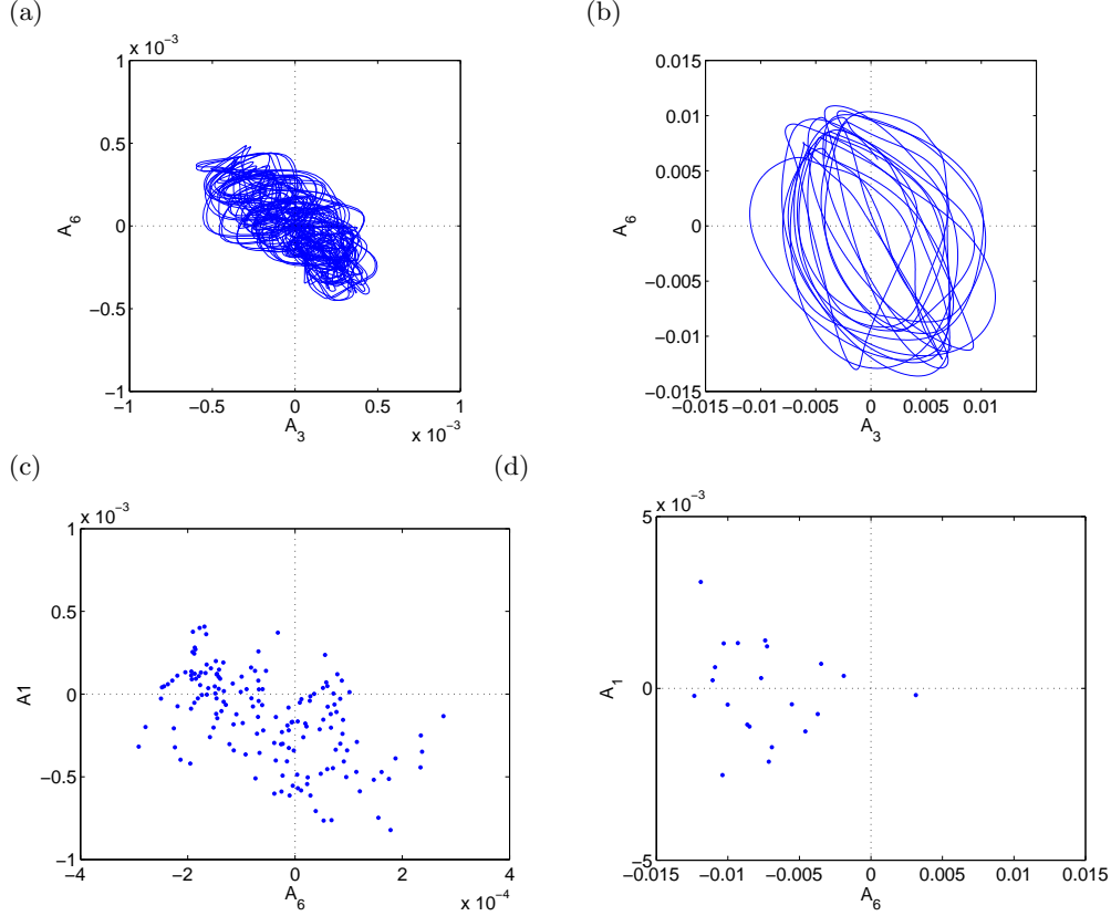
FIGURE 15. Phase portraits and Poincaré sections in the m = 3 regime: (a) Phase portrait of the amplitude of A_6 against A_3 for Ta = 2.0 \times 10^6 , (b) Phase portrait for Ta = 3.25 \times 10^6 ; (c) Poincaré section at A_3 = 0 showing A_1 against A_6 for Ta = 2.0 \times 10^6 . (d) Poincaré section as (c) but for Ta = 3.25 \times 10^6 .
