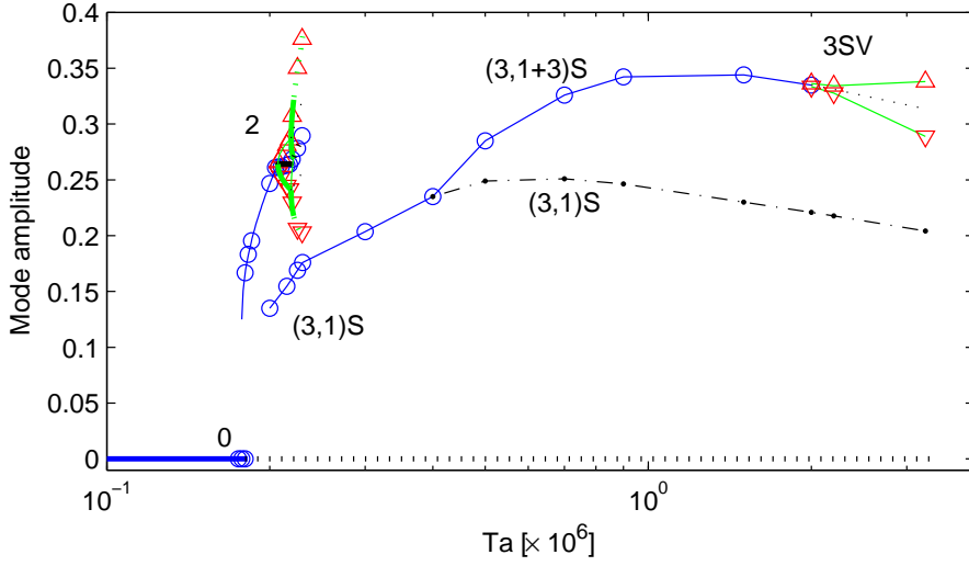
FIGURE 13. The amplitude of the m = 3 solutions against the Taylor number. The solid line and circles show the sum of the first three radial modes of the azimuthal mode m = 3 , while the dash-dotted line only shows the contribution of the first radial mode. For the vacillating flows, the mean amplitude is given by the dotted lines, and the amplitude extrema are shown by the solid lines and triangles. To put the m = 3 solutions into context, the transition from axisymmetric flow and the m = 2 solutions, shown in Figure 3 are reproduced.
