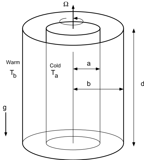
FIGURE 1. Schematic diagram of the baroclinic annulus.
