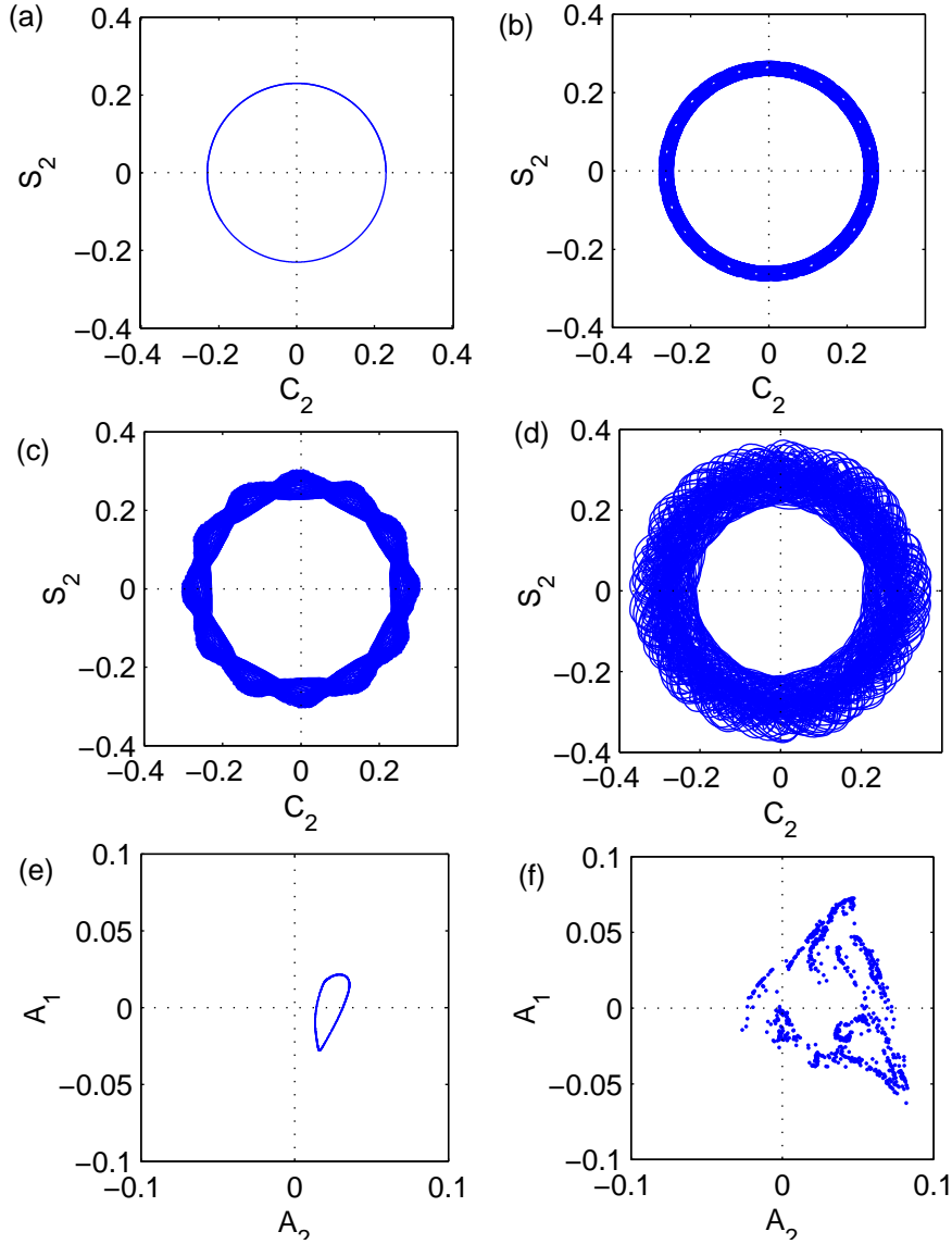
FIGURE 8. Phase space representations of: (a) a steady 2S ( Ta = 200,000 ), (b) a 2AV ( Ta = 215,000 ), (c) a quasi-periodic 2MAV ( Ta = 220,000 ), and (d) a chaotic 2MAV ( Ta = 229,250 ). The phase space diagrams show the time series of the sine component against that of the cosine component of mode m = 2 . Panels (e) and (f) show Poincaré sections of the amplitudes of m = 1 against m = 2 where m = 4 is zero, after the mean amplitudes had been subtracted.
