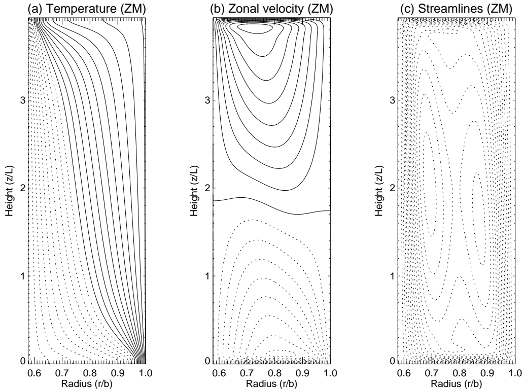
FIGURE 6. Zonal mean fields at Ta = 200,000 using air as the working fluid. (a) Temperature (contour interval = 0.1, normalised to an imposed temperature difference of \pm 1.0 ), (b) zonal velocity V_\phi (contour interval = 0.25) and (c) meridional stream function (contour interval = 0.01).
