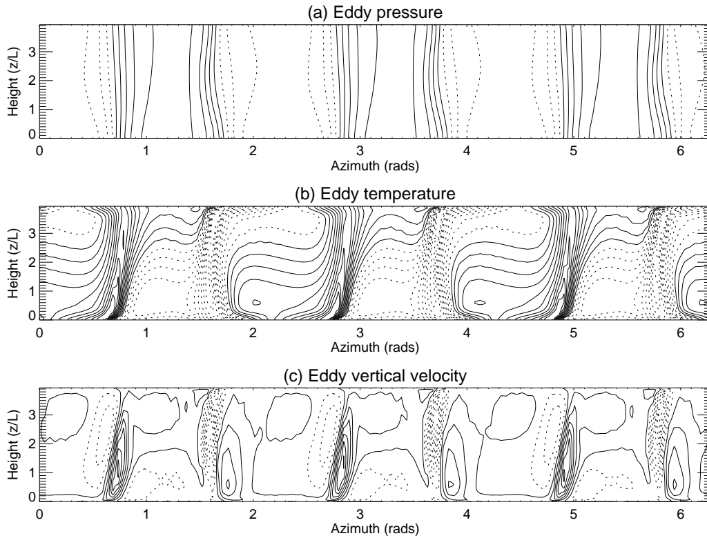
FIGURE 11. Azimuth-height maps of eddy fields (with azimuthal flow removed) in a typical simulation of the wave-3 flow at Ta = 1.5 \times 10^6 using air as the working fluid. (a) Pressure (contour interval = 0.25 dimensionless units), (b) Temperature T (contour interval = 0.05, normalised to an imposed temperature difference of \pm 1.0 ) and (c) Vertical velocity (contour interval = 0.5 dimensionless units).
