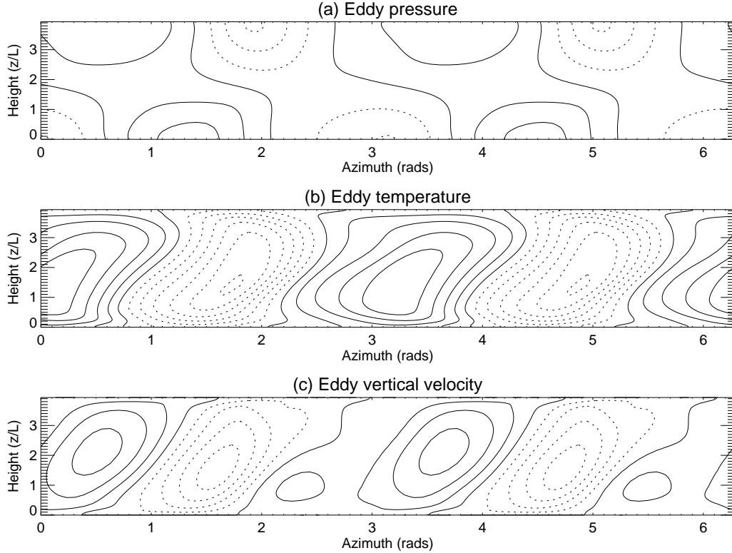
FIGURE 7. Azimuth-height maps of eddy fields (with azimuthal flow removed) in a typical simulation of a 2S flow at Ta = 200,000 using air as the working fluid. (a) Pressure (contour interval = 0.05 dimensionless units), (b) Temperature T (contour interval = 0.05, normalised to an imposed temperature difference of \pm 1.0 ) and (c) Vertical velocity (contour interval = 0.1 dimensionless units).
